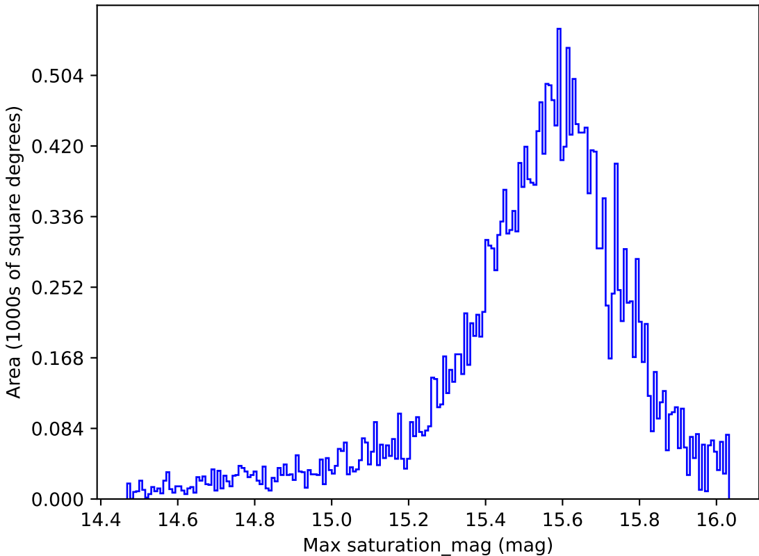
noroll_mjdp180_v3.4_10yrs All sky i band: Max saturation_mag
