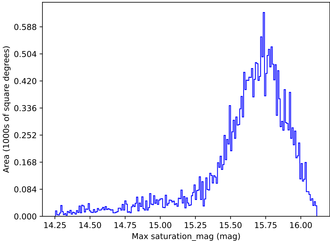
noroll_mjdp180_v3.4_10yrs All sky g band: Max saturation_mag
