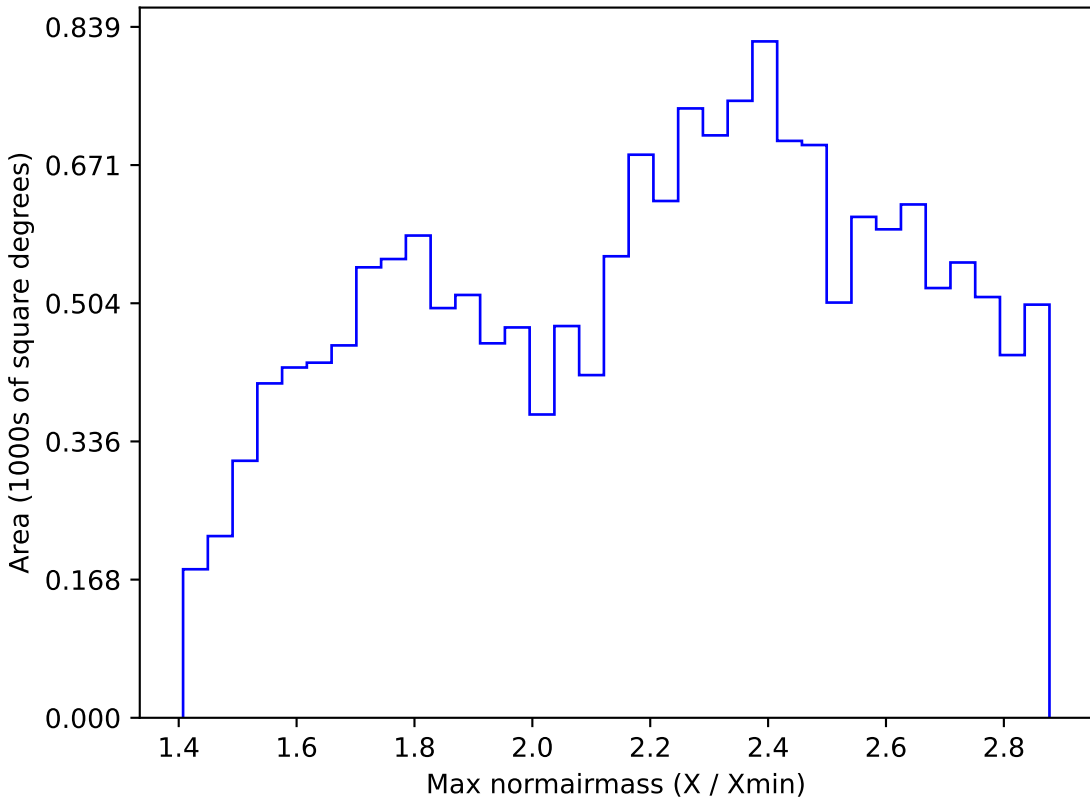
noroll_mjdp180_v3.4_10yrs WFD z band: Max normairmass
