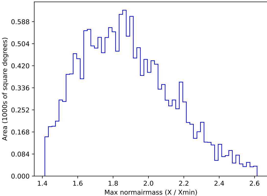
noroll_mjdp180_v3.4_10yrs WFD y band: Max normairmass
