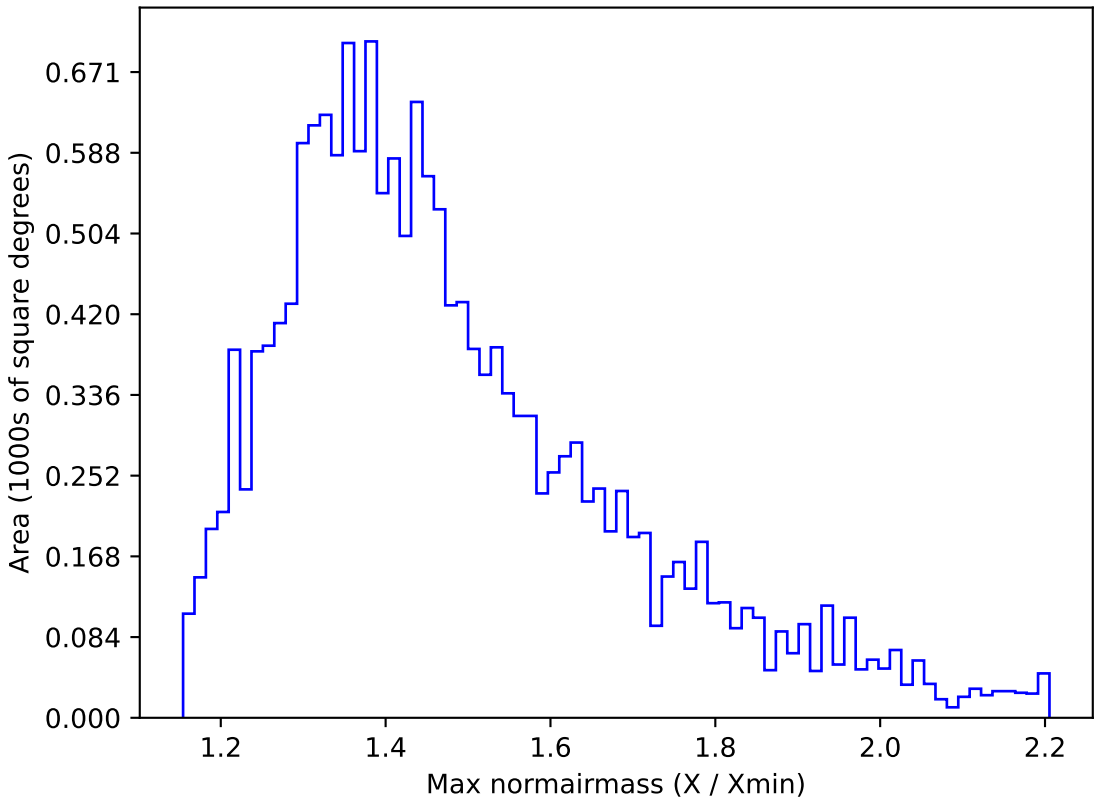
noroll_mjdp180_v3.4_10yrs WFD u band: Max normairmass
