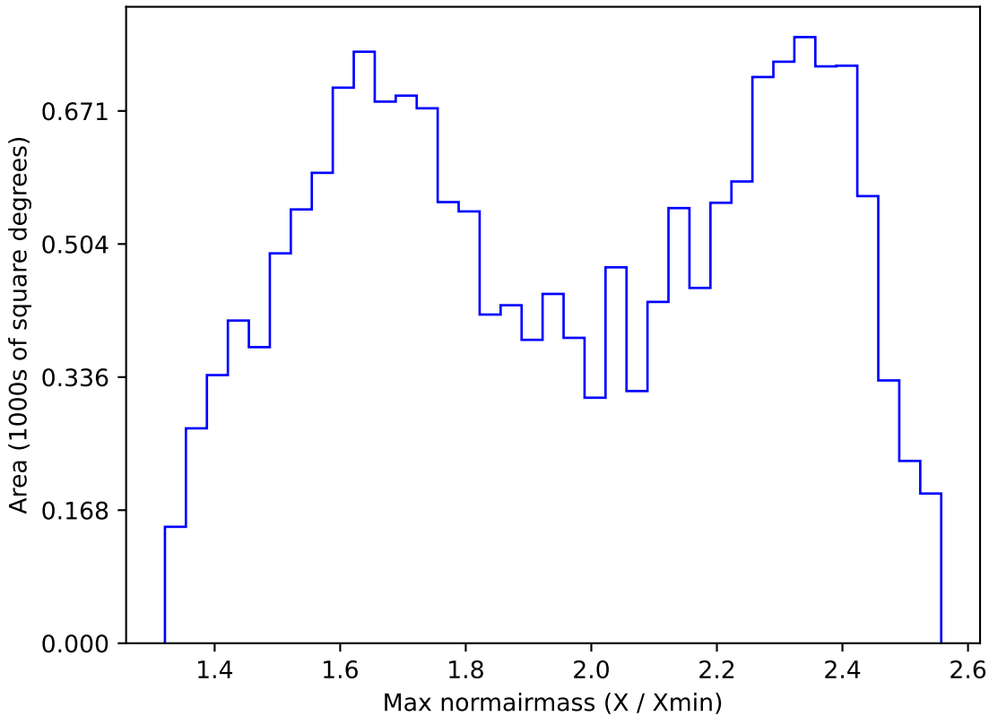
noroll_mjdp180_v3.4_10yrs WFD r band: Max normairmass
