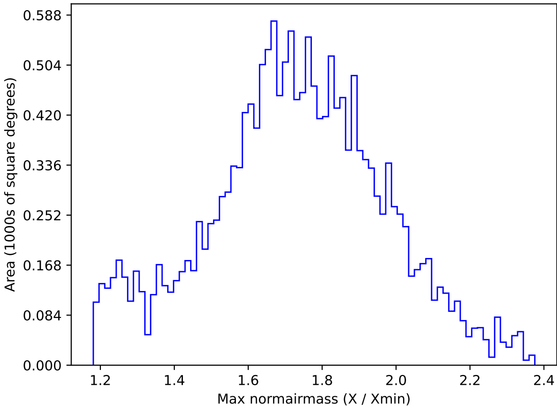
noroll_mjdp180_v3.4_10yrs WFD g band: Max normairmass
