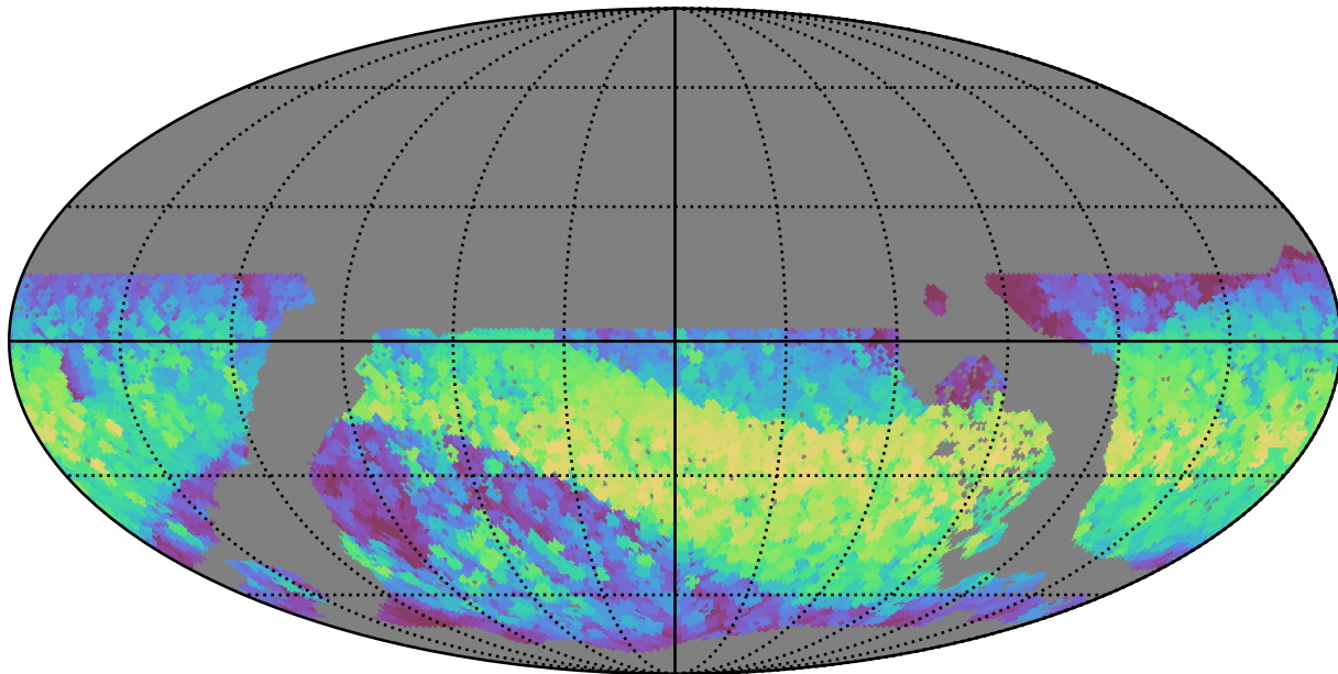
noroll_mjdp180_v3.4_10yrs WFD all bands: Max normairmass
