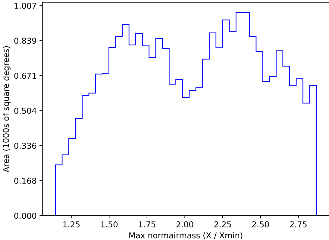
noroll_mjdp180_v3.4_10yrs All sky z band: Max normairmass
