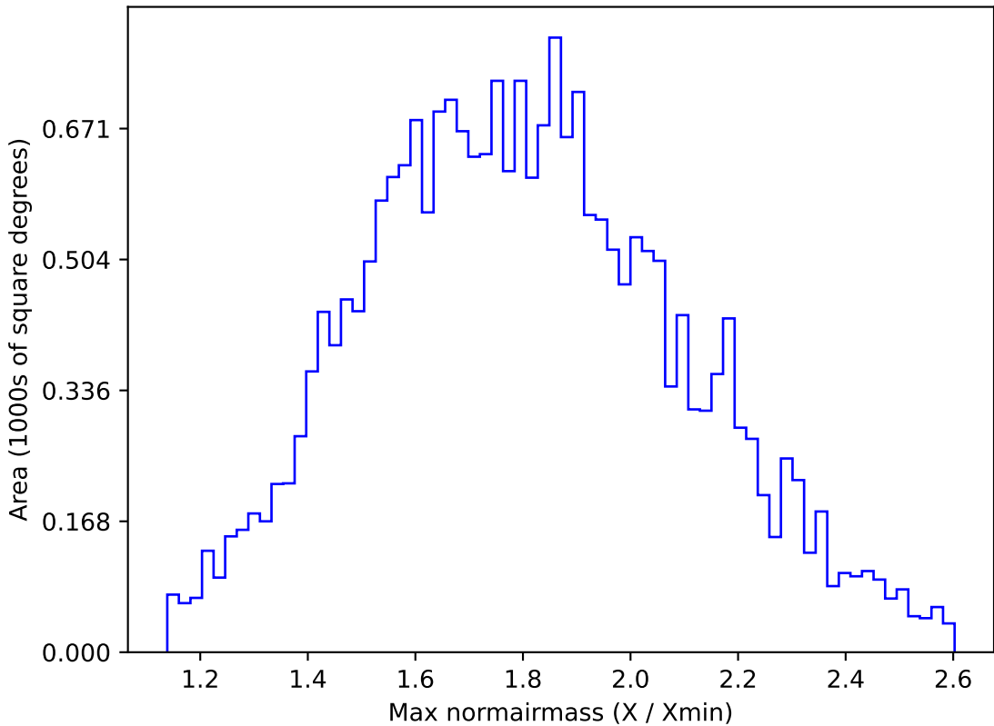
noroll_mjdp180_v3.4_10yrs All sky y band: Max normairmass
