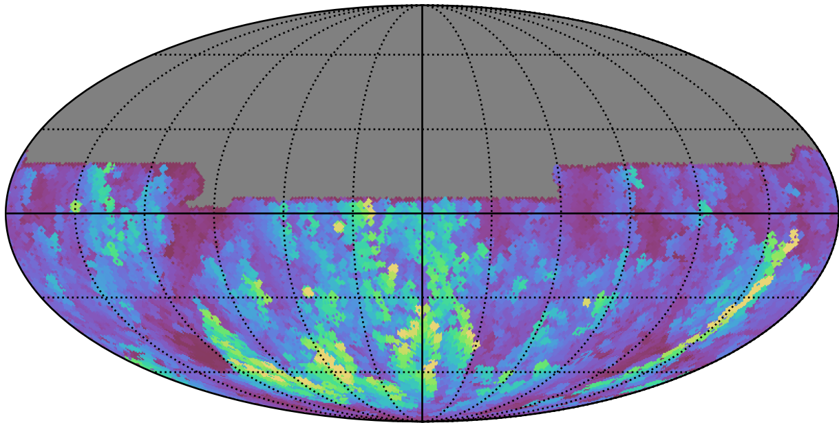
noroll_mjdp180_v3.4_10yrs All sky u band: Max normairmass
