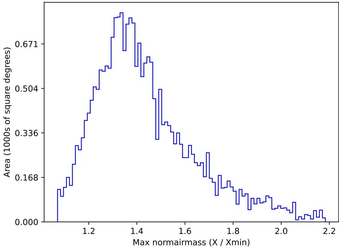
noroll_mjdp180_v3.4_10yrs All sky u band: Max normairmass
