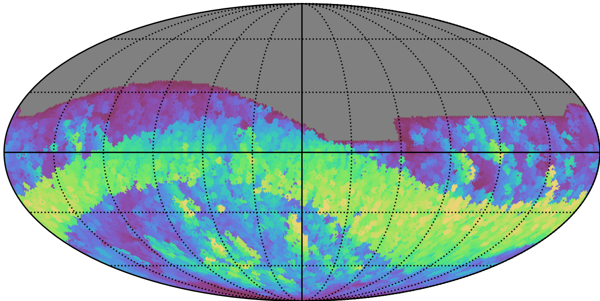
noroll_mjdp180_v3.4_10yrs All sky r band: Max normairmass
