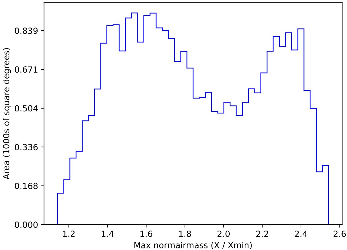
noroll_mjdp180_v3.4_10yrs All sky r band: Max normairmass
