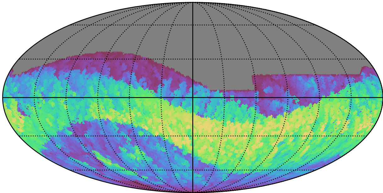
noroll_mjdp180_v3.4_10yrs All sky i band: Max normairmass
