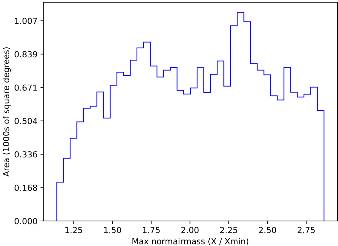
noroll_mjdp180_v3.4_10yrs All sky i band: Max normairmass
