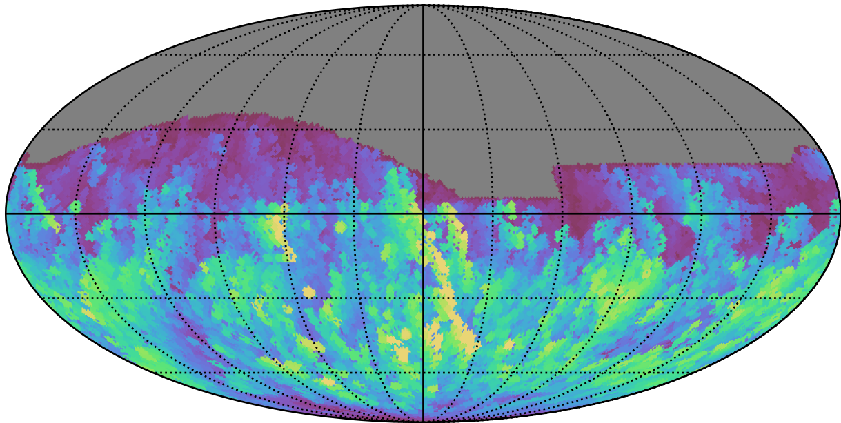
noroll_mjdp180_v3.4_10yrs All sky g band: Max normairmass
