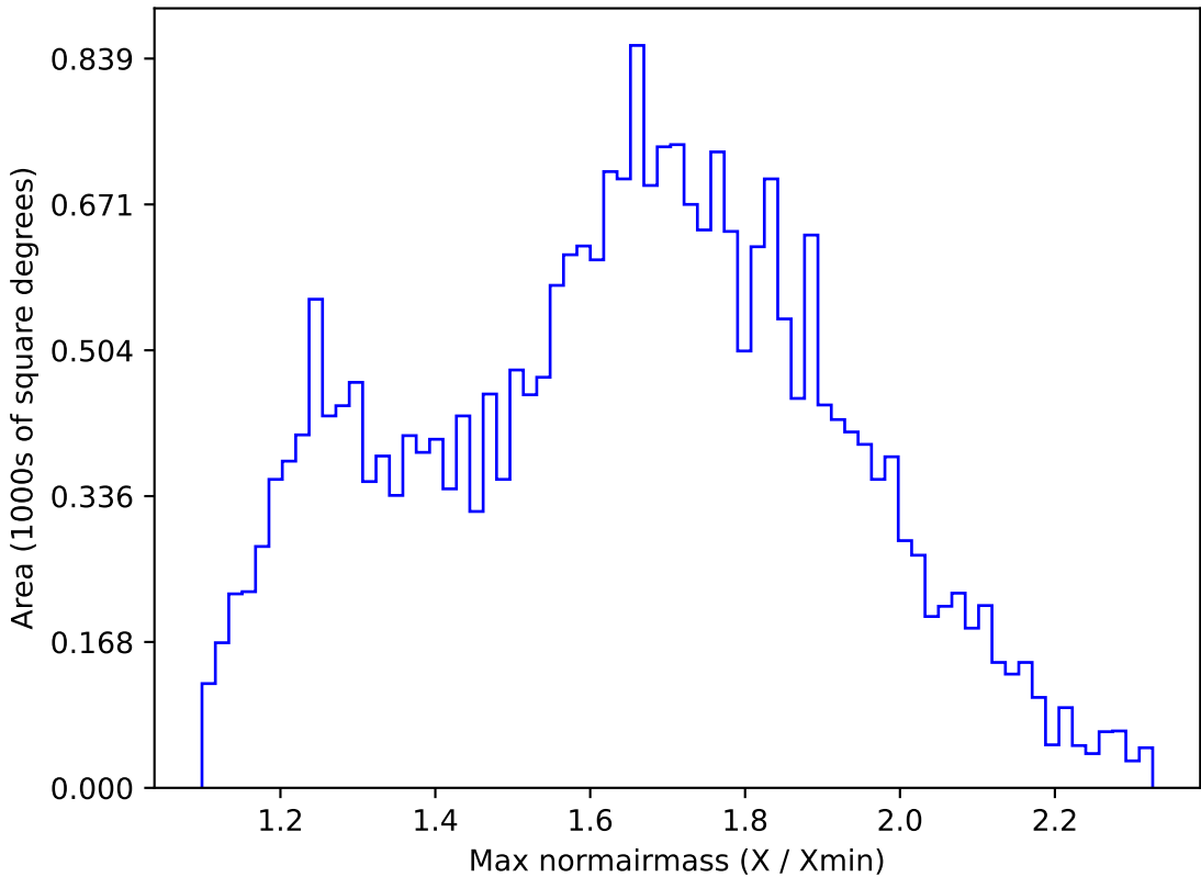
noroll_mjdp180_v3.4_10yrs All sky g band: Max normairmass
