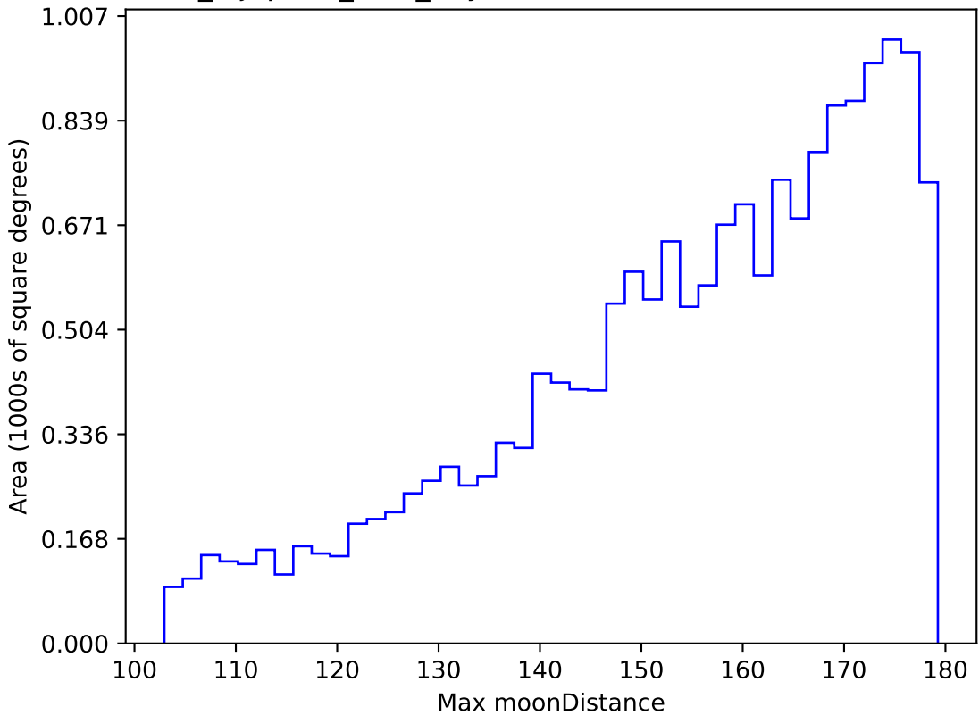
noroll_mjdp180_v3.4_10yrs WFD z band: Max moonDistance
