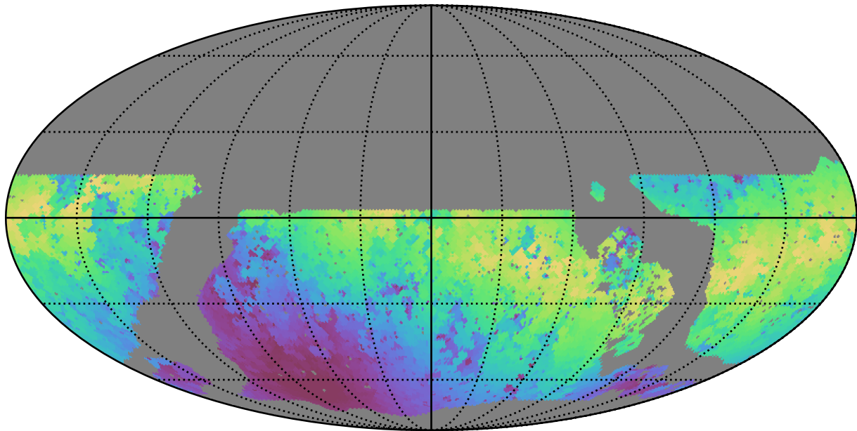
noroll_mjdp180_v3.4_10yrs WFD y band: Max moonDistance
