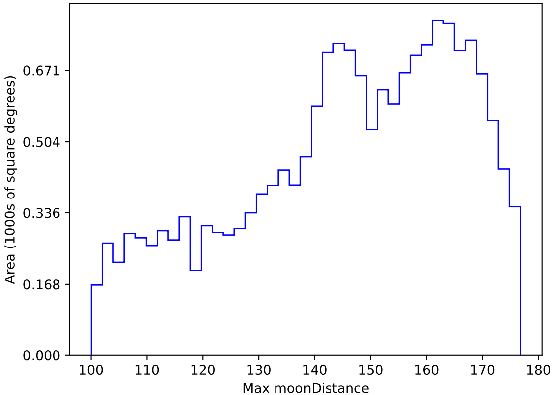
noroll_mjdp180_v3.4_10yrs WFD y band: Max moonDistance
