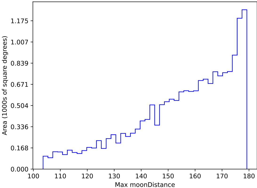
noroll_mjdp180_v3.4_10yrs WFD i band: Max moonDistance
