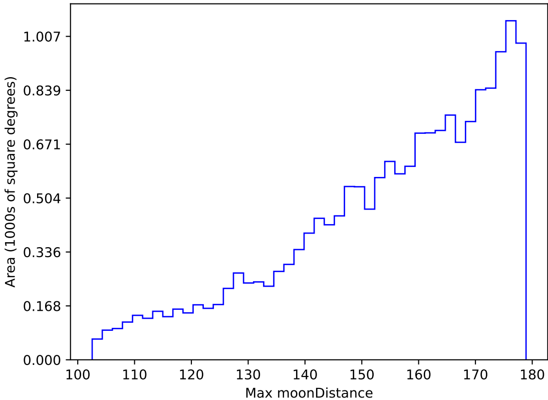
noroll_mjdp180_v3.4_10yrs WFD g band: Max moonDistance
