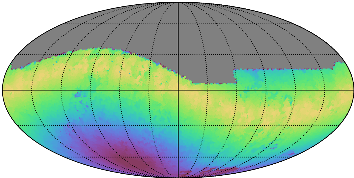
noroll_mjdp180_v3.4_10yrs All sky z band: Max moonDistance
