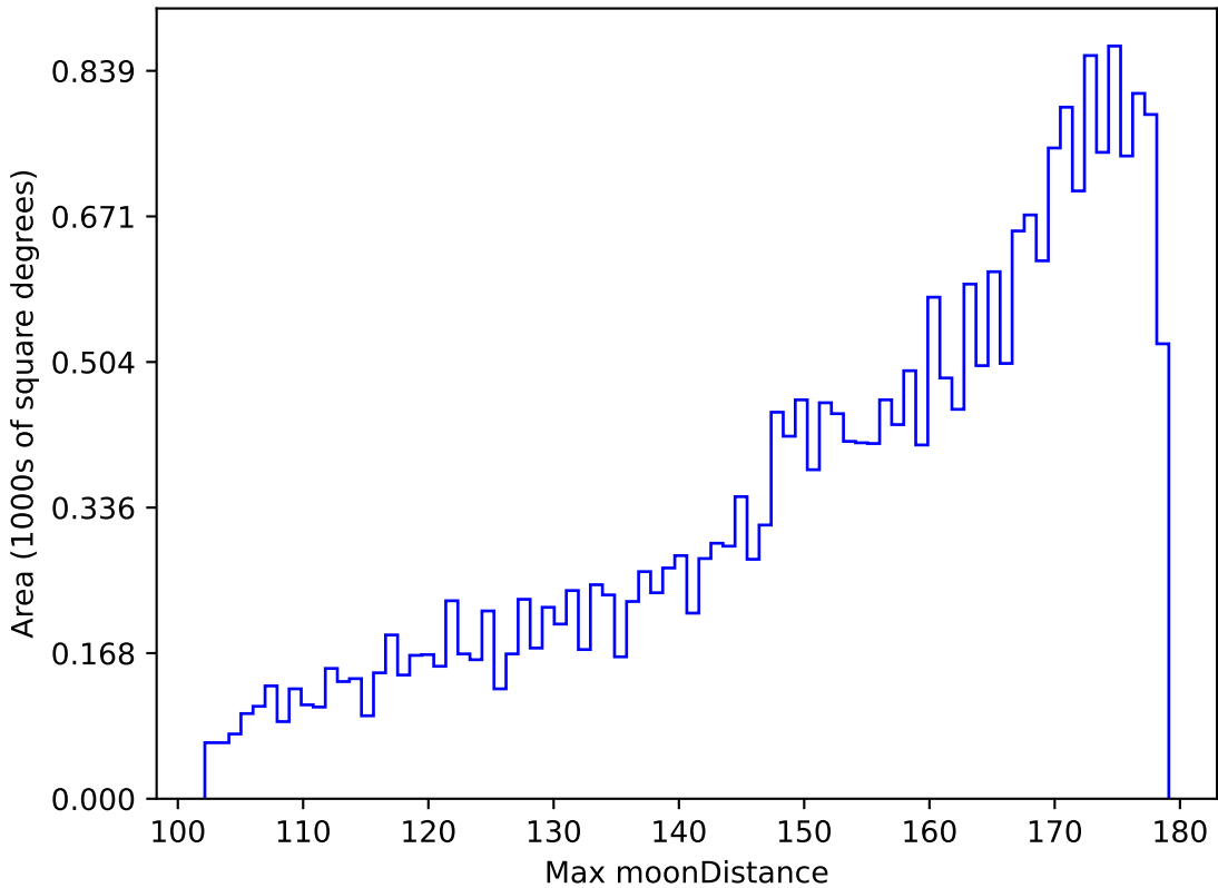
noroll_mjdp180_v3.4_10yrs All sky z band: Max moonDistance
