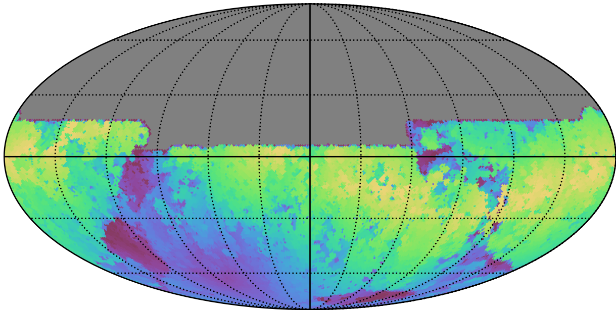
noroll_mjdp180_v3.4_10yrs All sky y band: Max moonDistance
