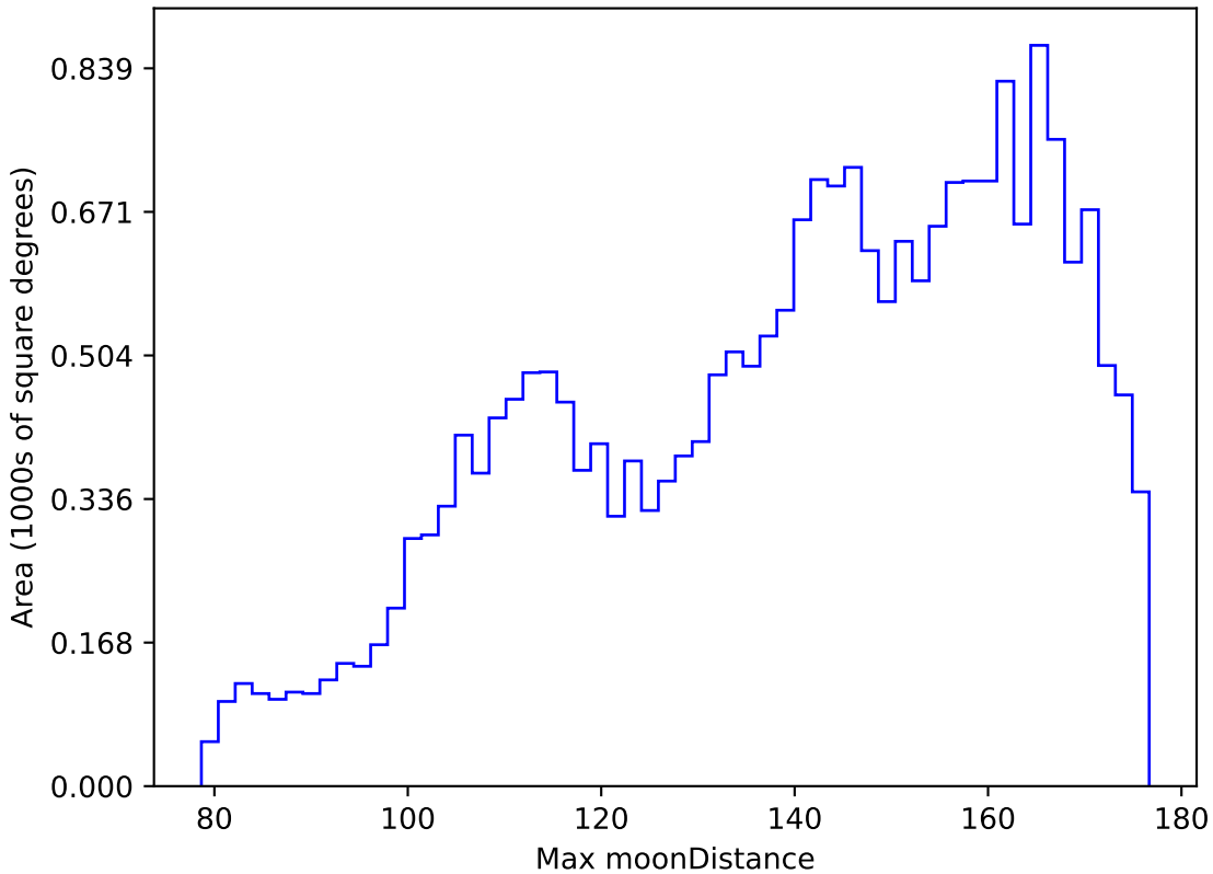
noroll_mjdp180_v3.4_10yrs All sky y band: Max moonDistance
