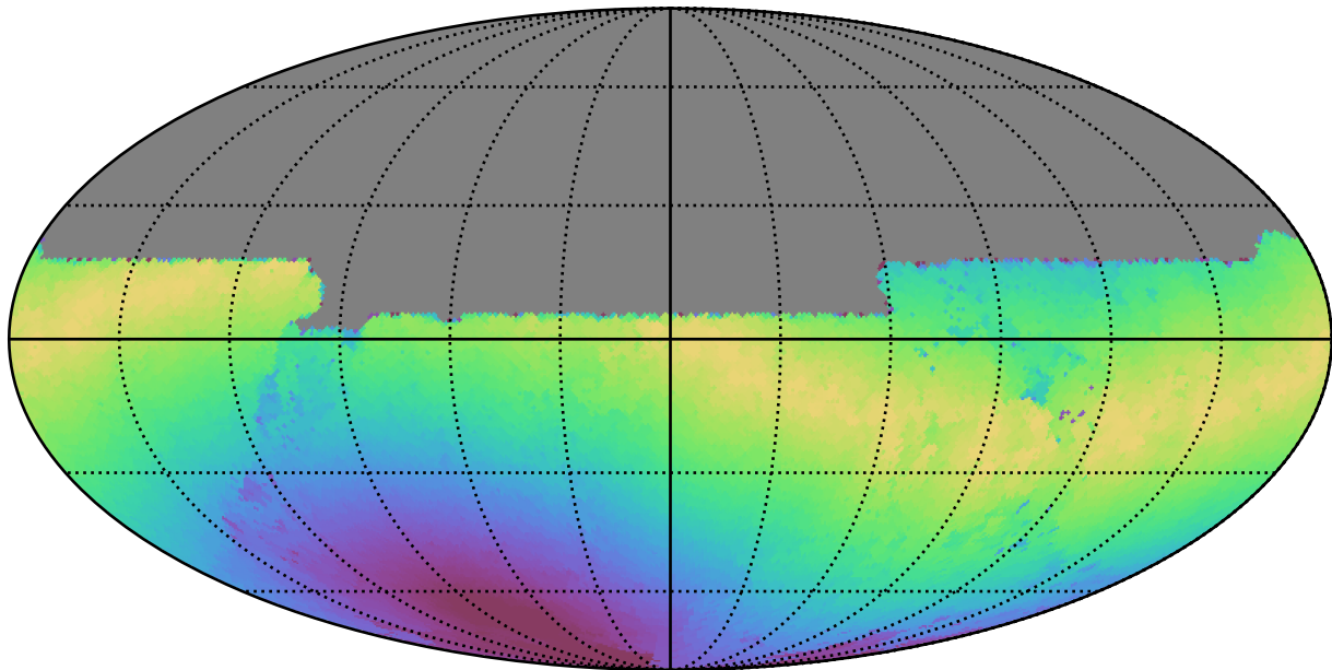
noroll_mjdp180_v3.4_10yrs All sky u band: Max moonDistance
