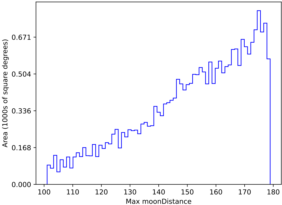
noroll_mjdp180_v3.4_10yrs All sky u band: Max moonDistance
