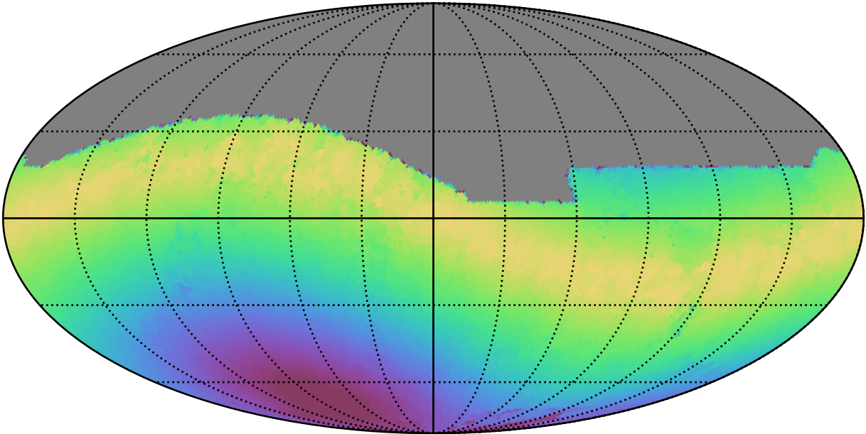
noroll_mjdp180_v3.4_10yrs All sky r band: Max moonDistance
