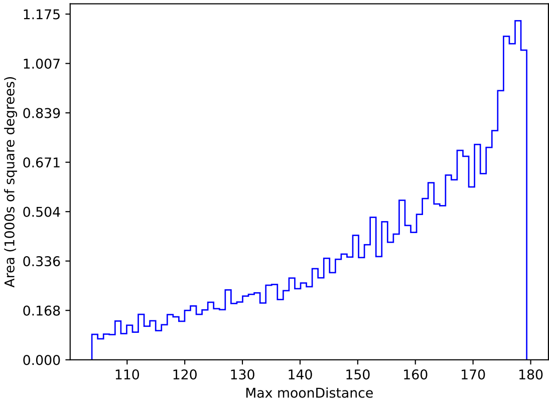
noroll_mjdp180_v3.4_10yrs All sky r band: Max moonDistance
