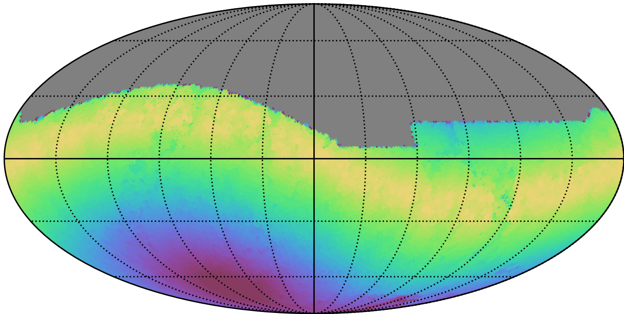
noroll_mjdp180_v3.4_10yrs All sky i band: Max moonDistance
