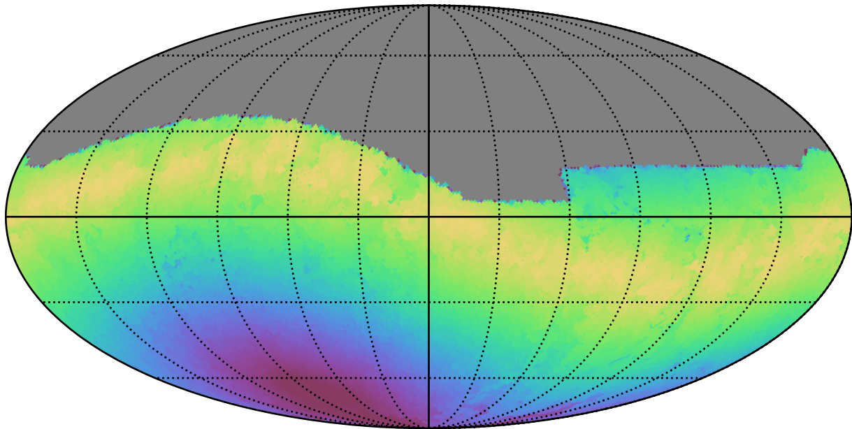
noroll_mjdp180_v3.4_10yrs All sky g band: Max moonDistance
