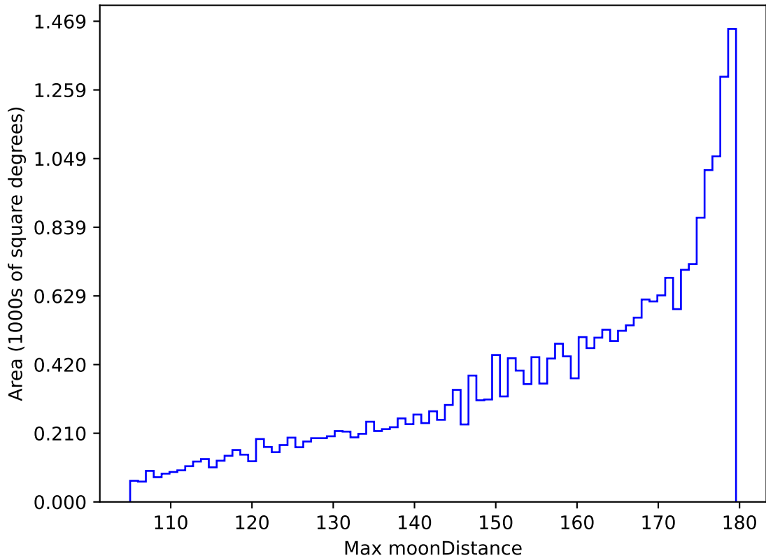
noroll_mjdp180_v3.4_10yrs All sky all bands: Max moonDistance
