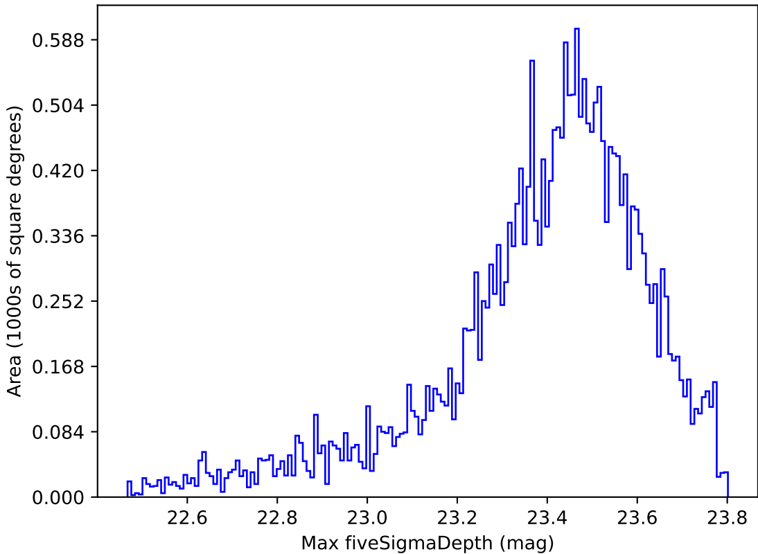
noroll_mjdp180_v3.4_10yrs Yr 1 z band: Max fiveSigmaDepth
