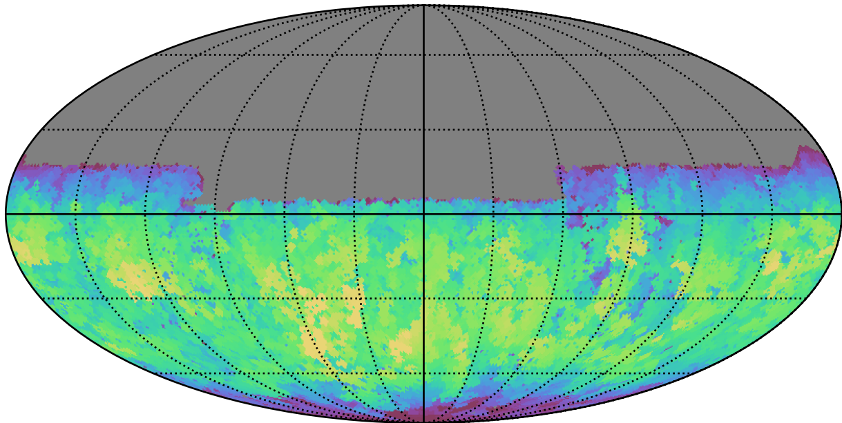
noroll_mjdp180_v3.4_10yrs Yr 1 y band: Max fiveSigmaDepth
