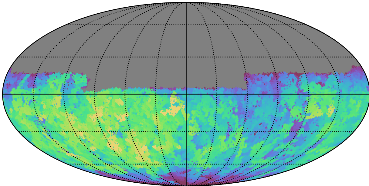
noroll_mjdp180_v3.4_10yrs Yr 1 u band: Max fiveSigmaDepth
