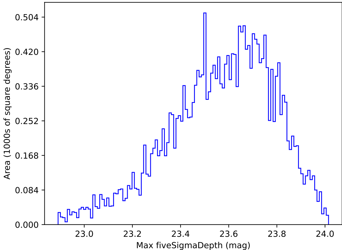
noroll_mjdp180_v3.4_10yrs Yr 1 u band: Max fiveSigmaDepth
