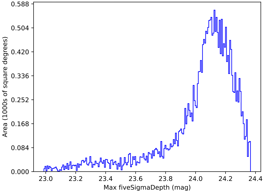
noroll_mjdp180_v3.4_10yrs Yr 1 i band: Max fiveSigmaDepth
