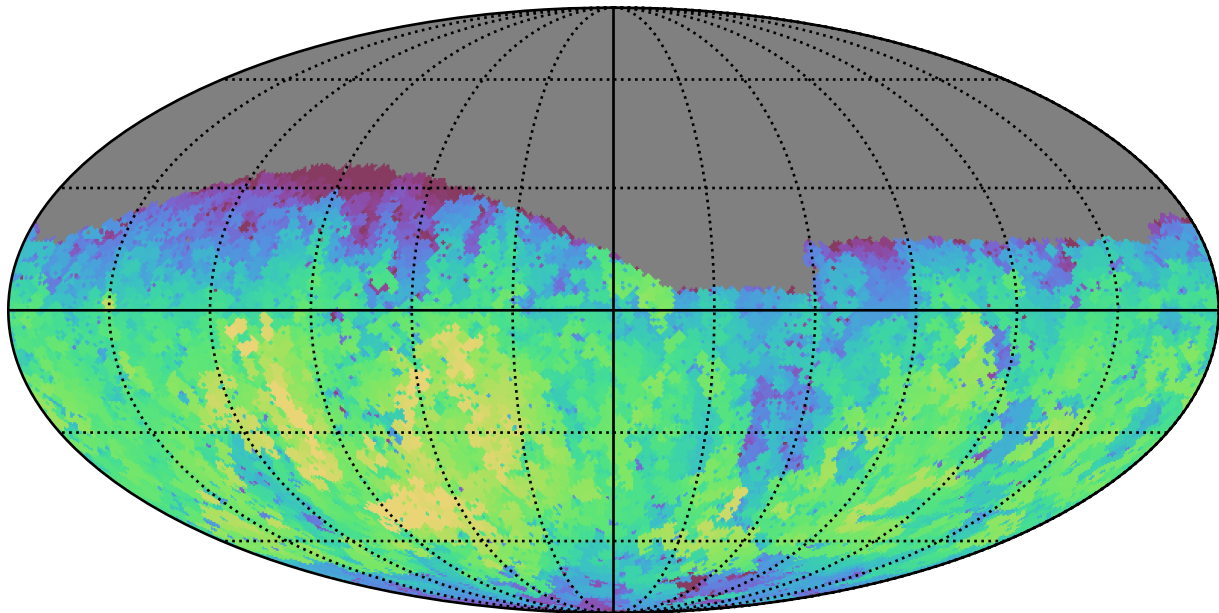
noroll_mjdp180_v3.4_10yrs Yr 1 g band: Max fiveSigmaDepth
