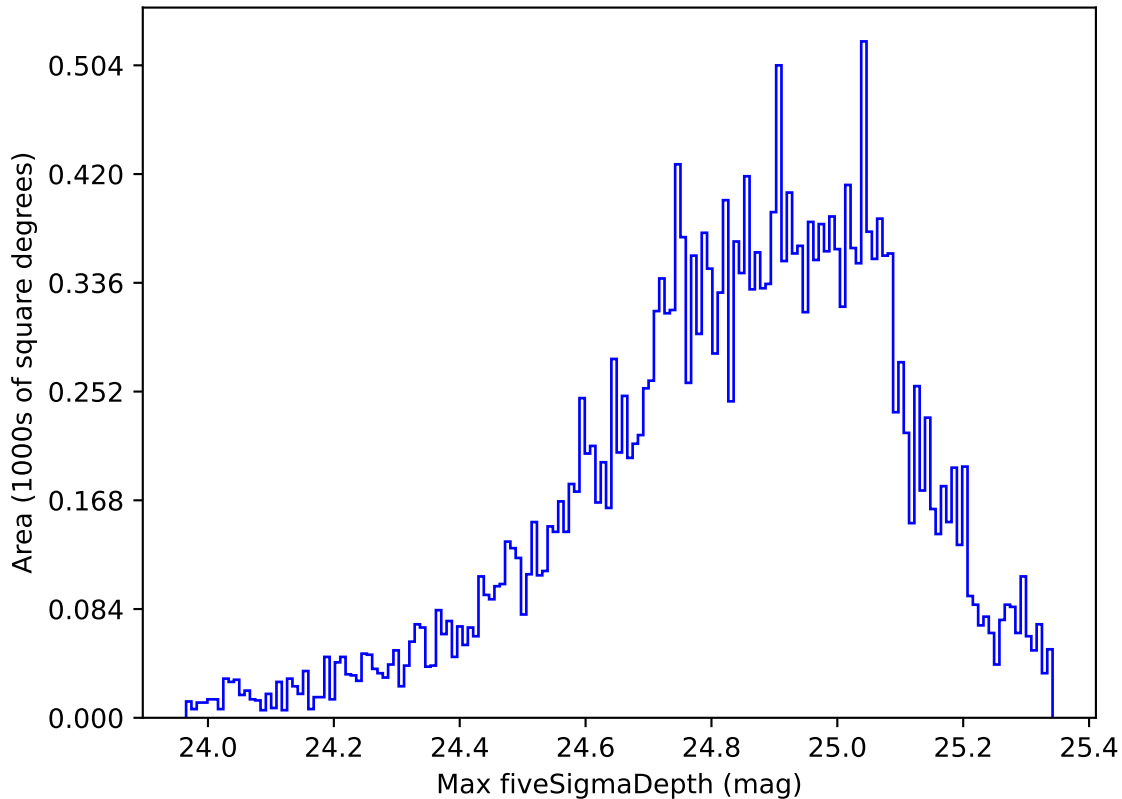
noroll_mjdp180_v3.4_10yrs Yr 1 g band: Max fiveSigmaDepth
