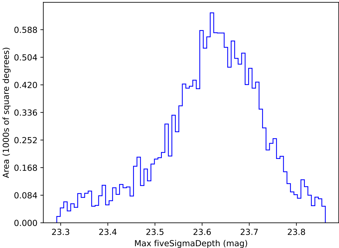
noroll_mjdp180_v3.4_10yrs WFD z band: Max fiveSigmaDepth
