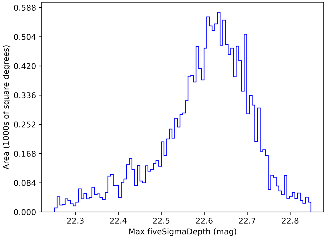
noroll_mjdp180_v3.4_10yrs WFD y band: Max fiveSigmaDepth
