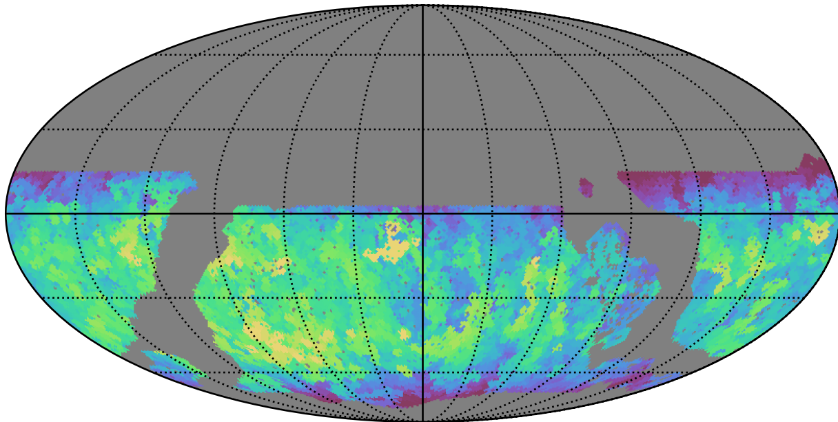
noroll_mjdp180_v3.4_10yrs WFD u band: Max fiveSigmaDepth
