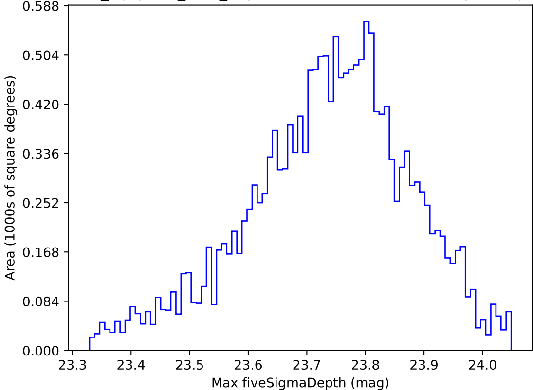
noroll_mjdp180_v3.4_10yrs WFD u band: Max fiveSigmaDepth
