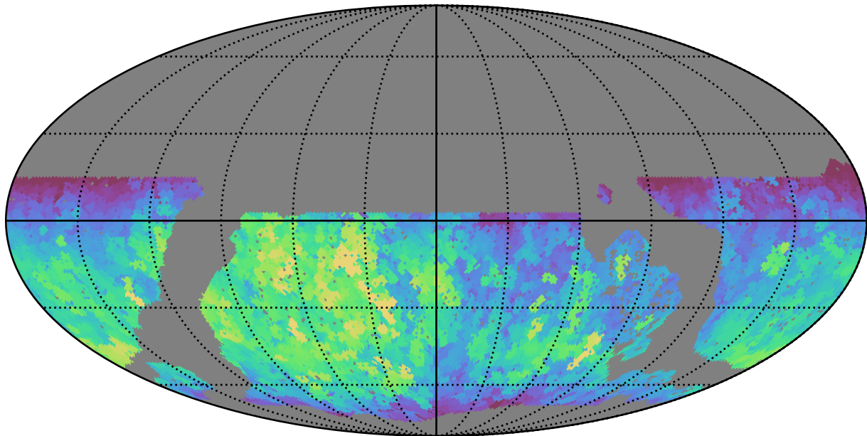
noroll_mjdp180_v3.4_10yrs WFD r band: Max fiveSigmaDepth
