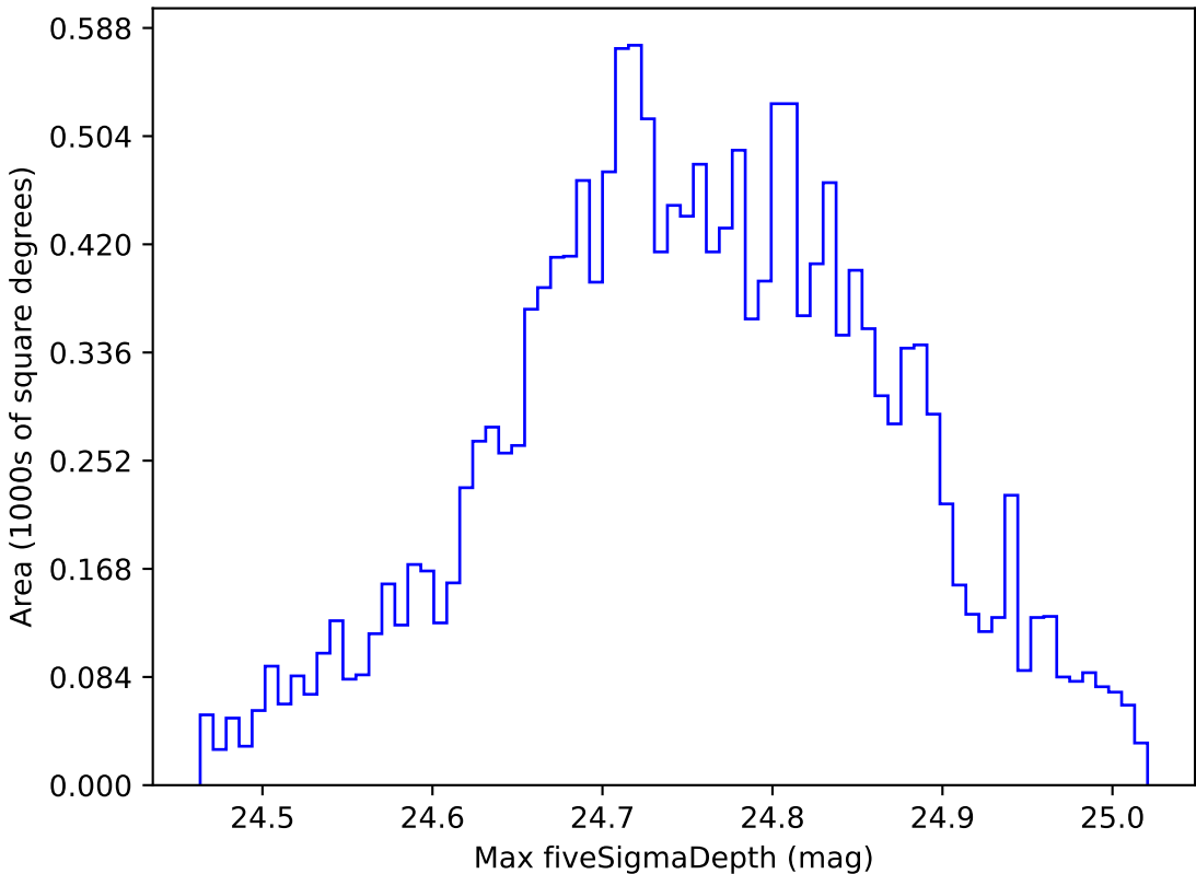
noroll_mjdp180_v3.4_10yrs WFD r band: Max fiveSigmaDepth
