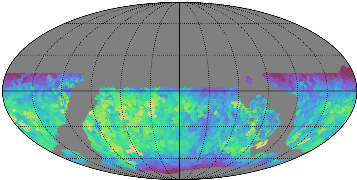
noroll_mjdp180_v3.4_10yrs WFD i band: Max fiveSigmaDepth
