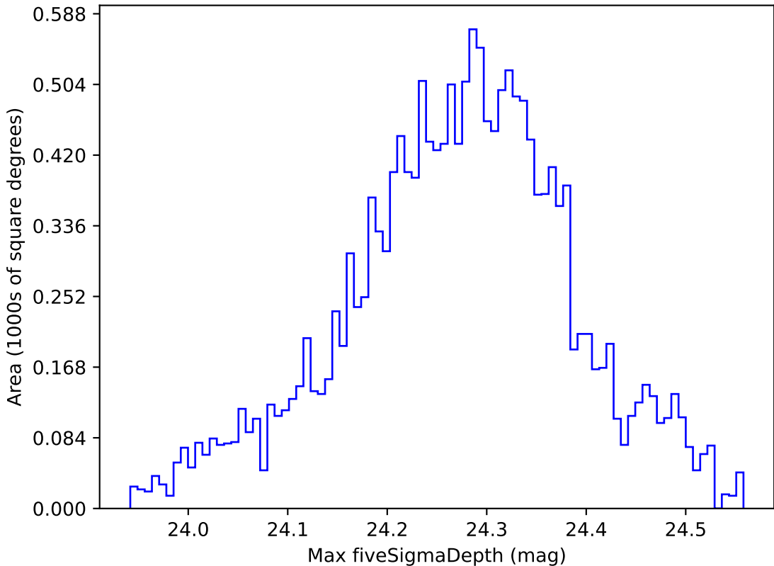
noroll_mjdp180_v3.4_10yrs WFD i band: Max fiveSigmaDepth
