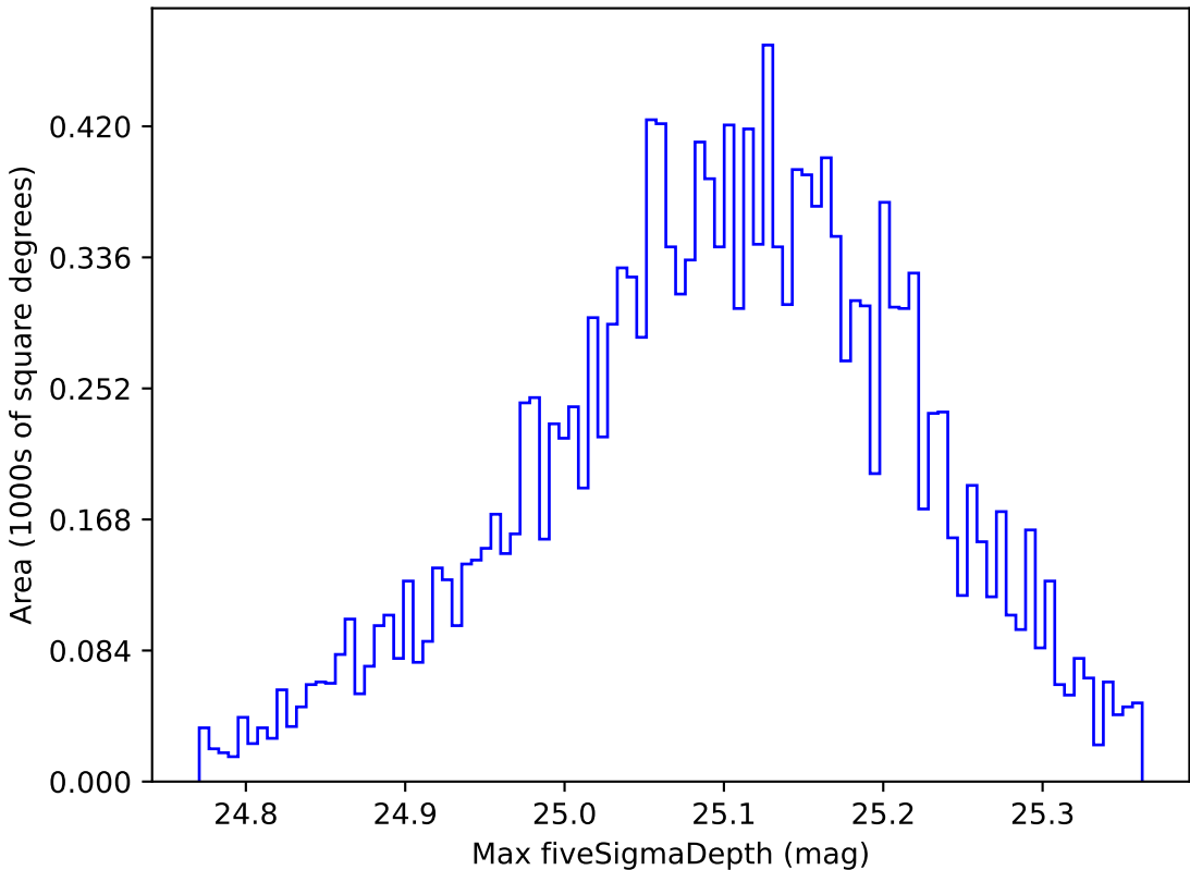
noroll_mjdp180_v3.4_10yrs WFD g band: Max fiveSigmaDepth
